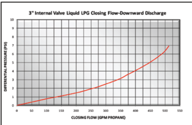
MEC Excelerator ™ 3" Flanged Internal Valves
