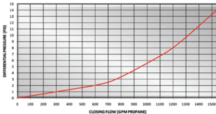
4" Internal Valve Liquid LPG Closing Flow-Downward Discharge
